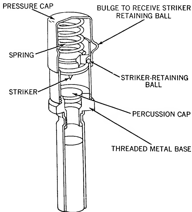
Figure 35. Soviet pressure fuze MV-5.
